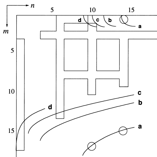
Fig. 7. A schematic projection onto the nm plane of the SmC phase domain (below N) for complexes Cu1- n.m . Contours of (a) T_{CN}/T_{NI}=1.00 , (b) 0.97, (c) 0.94, and (d) 0.91, estimated from the data reported to date, are given. Purely nematogenic homologues (as reported) are indicated by squaring their sites, and three circled homologues on curve (a) are pure smectogens.
